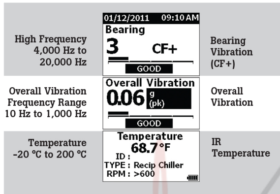
Sample measurement results screen indicating a four-level severity scale (Good, Satisfactory, Unsatisfactory, Unacceptable) for bearing and overall vibration
