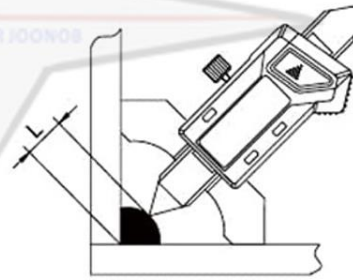
Fillet Weld Thickness
