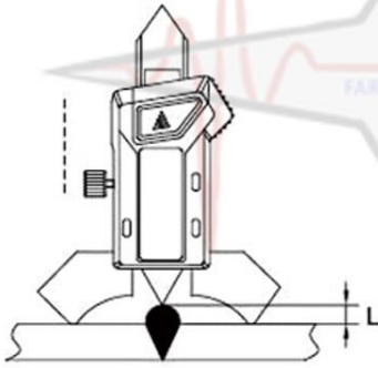
Weld Height
