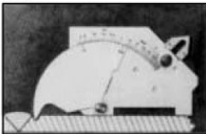
UNDERCUT
