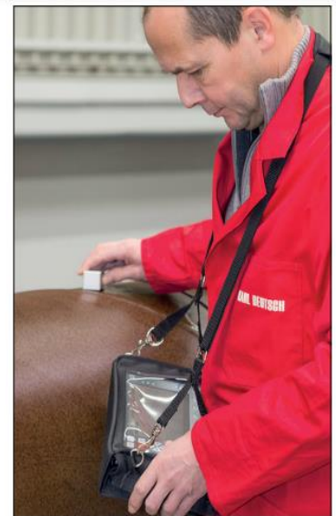
Mobile ultrasonic inspection with the ECHOGRAPH 1095 in the practical carrying case
